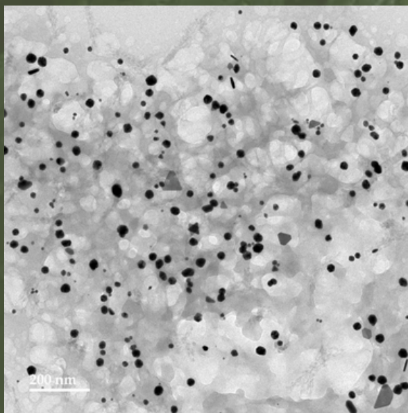
TEM Image of CNM-AU-00209
