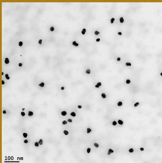
TEM Image of SGM-AU-00149
