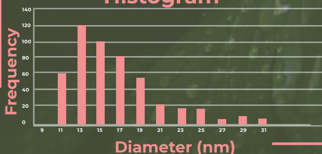
Histogram
