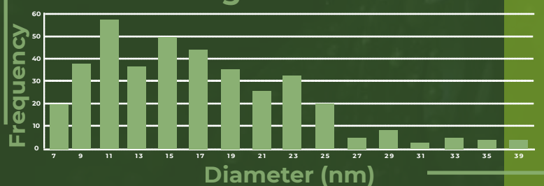
Histogram
