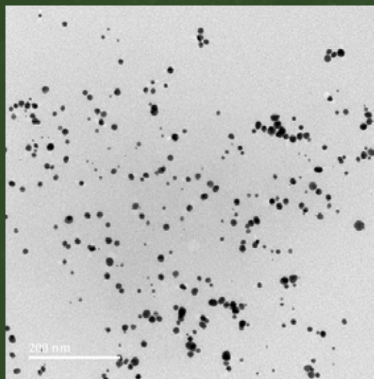
TEM Image of SFD-AU-00092
