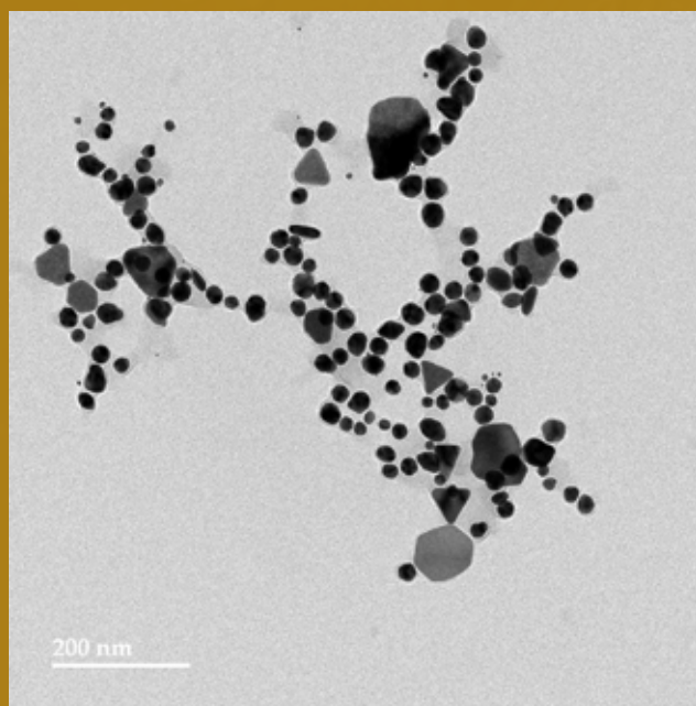
TEM Image of PSP-AU-00078
