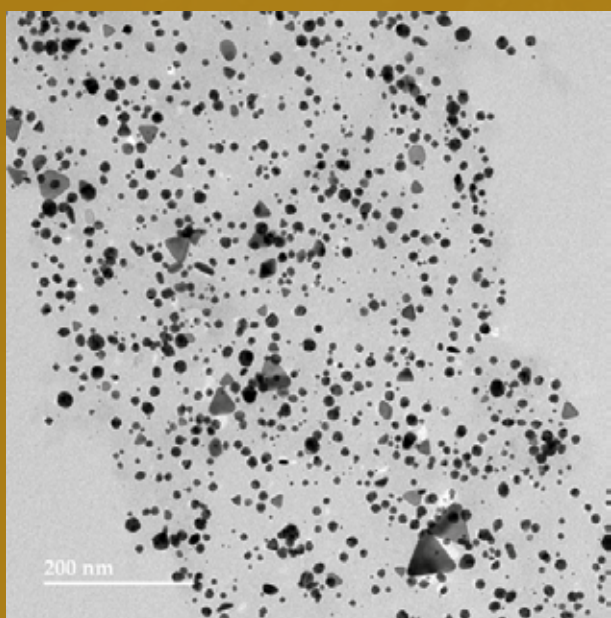
TEM Image of BAL-AU-00048
