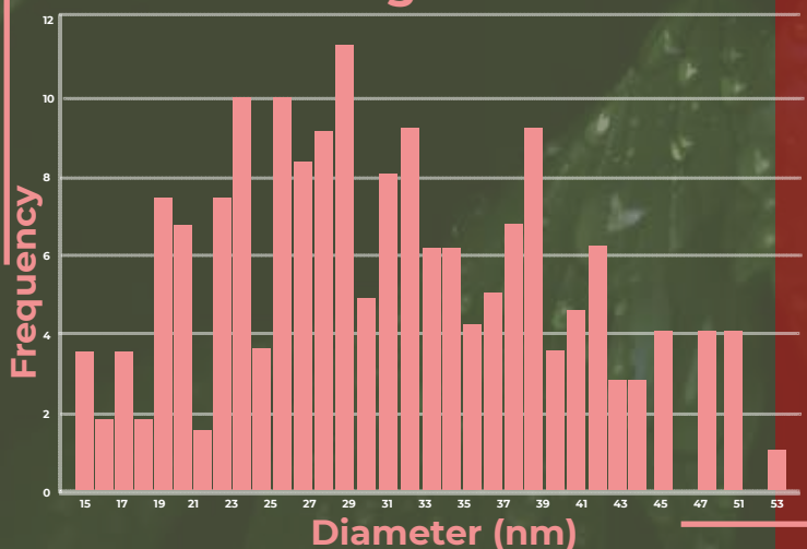
Histogram
