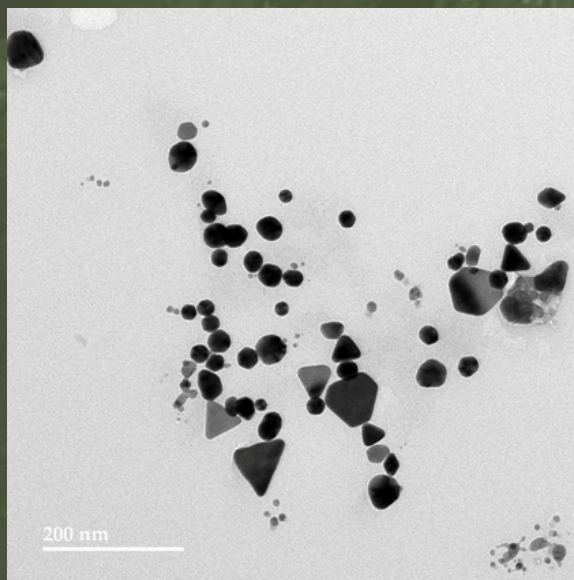
TEM Image of LON-AG-00268
