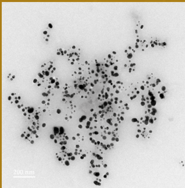
TEM Image of LDR-AG-00203
