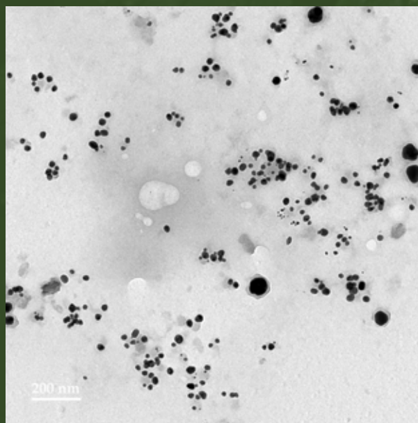
TEM Image of ARK-AG-00112
