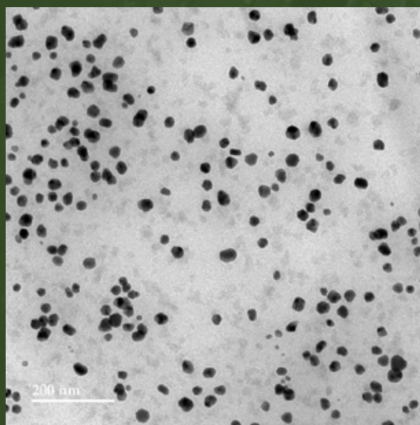
TEM Image of PLS-AG-00077
