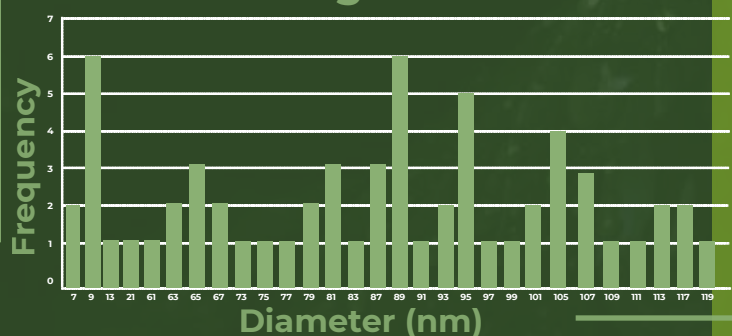
Histogram
